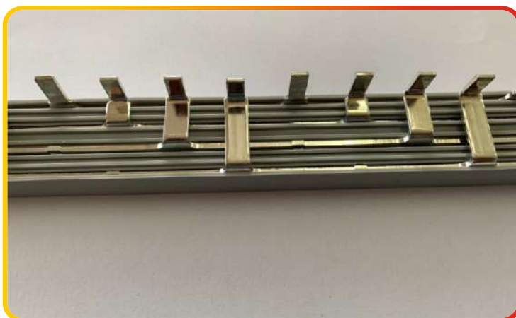
FOUR POLE SHORTING LINK BUSBAR
